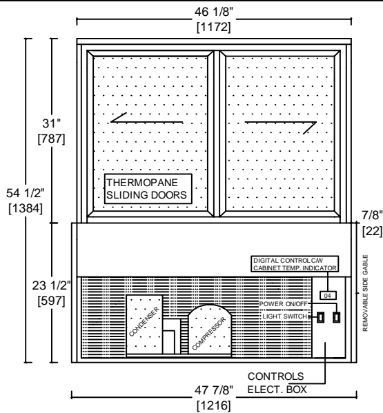
REAR VIEW 48" LONG UNIT SHOWN
